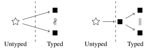
Figure 1: Inserting a type adaptor
