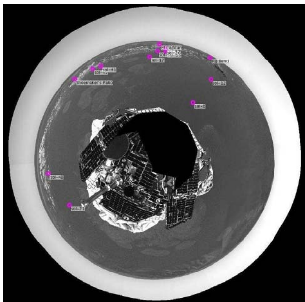
Fig. 3. Navcam polar-azimuthal mosaic view of Eagle Crater from the Opportunity rover taken prior to its egress from the lander. The image is annotated with various target locations denoting features of interest and locations where the rover traversed to following egress.
