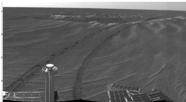
Fig. 2. Navcam cylindrical mosaic view from the Opportunity rover looking back after egress from Eagle Crater at Meridiani Planum.
